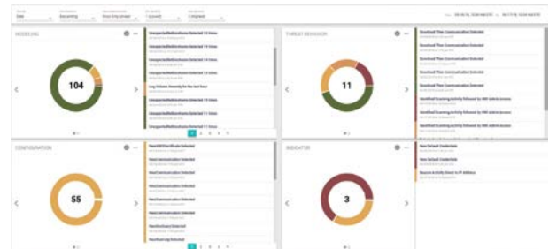
Figure 4: Detections Dashboard
